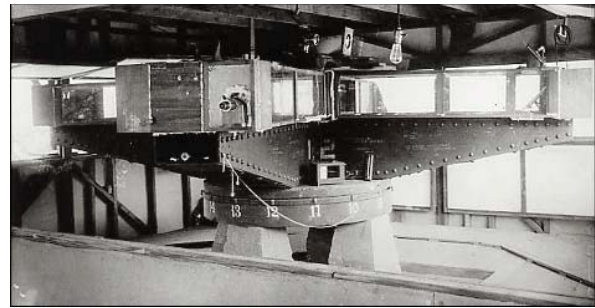
Fig. 3: Miller's interferometer with an effective arm length of L=32\text{m} achieved by multiple reflections. Used by Miller on Mt.Wilson to perform the 1925–1926 observations of absolute motion. The steel arms weighed 1200 kilograms and floated in a tank of 275 kilograms of Mercury. From Case Western Reserve University Archives.
